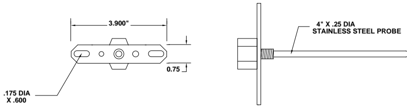
Duct/Immersion sensor shown without box.
